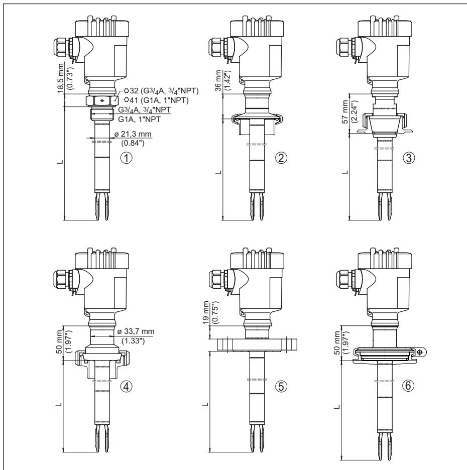
插图. 20: VEGASWING 63
