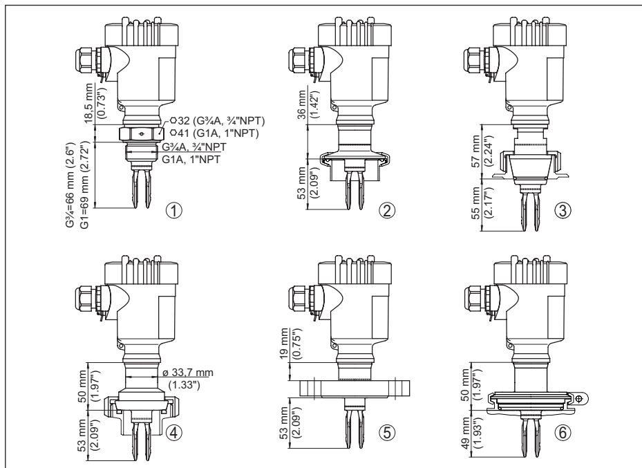
插图. 18: VEGASWING 61
