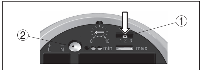
插图. 17: 补偿键
