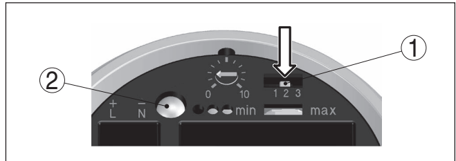
插图. 16: 补偿键
