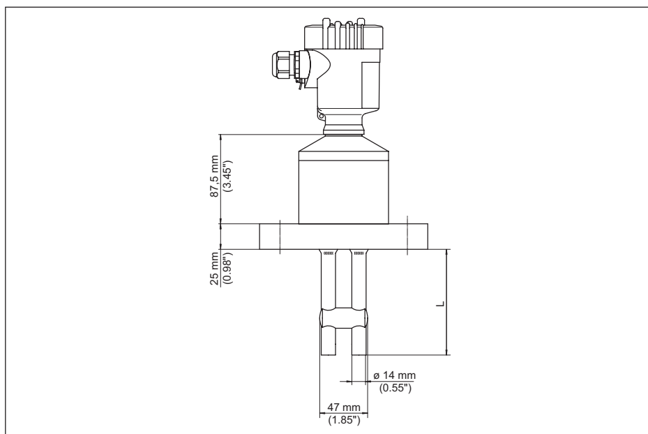
插图. 34: VEGACAL 69
