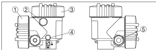
插图. 12: 双腔式外壳
