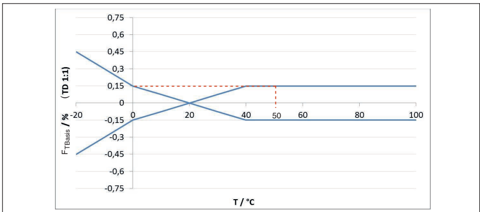
插图. 27: 为上例计算基本温度误差: F_{\text{Tbasis}} = \mathbf{0.15 \%}
